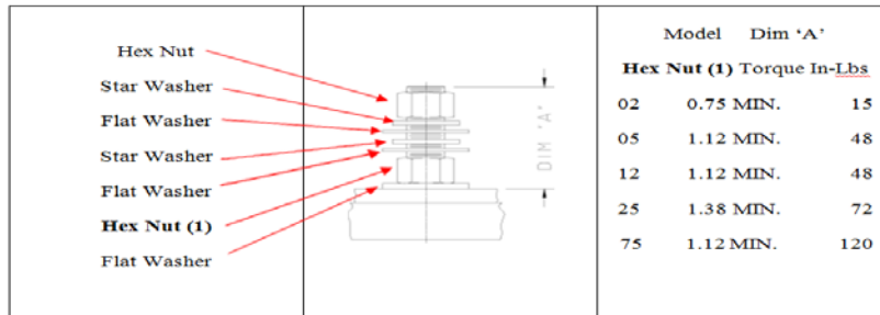
Figure A – Metallic Pump Grounding
