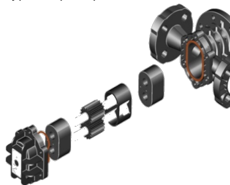
Figure 3 – KOPkit Components
