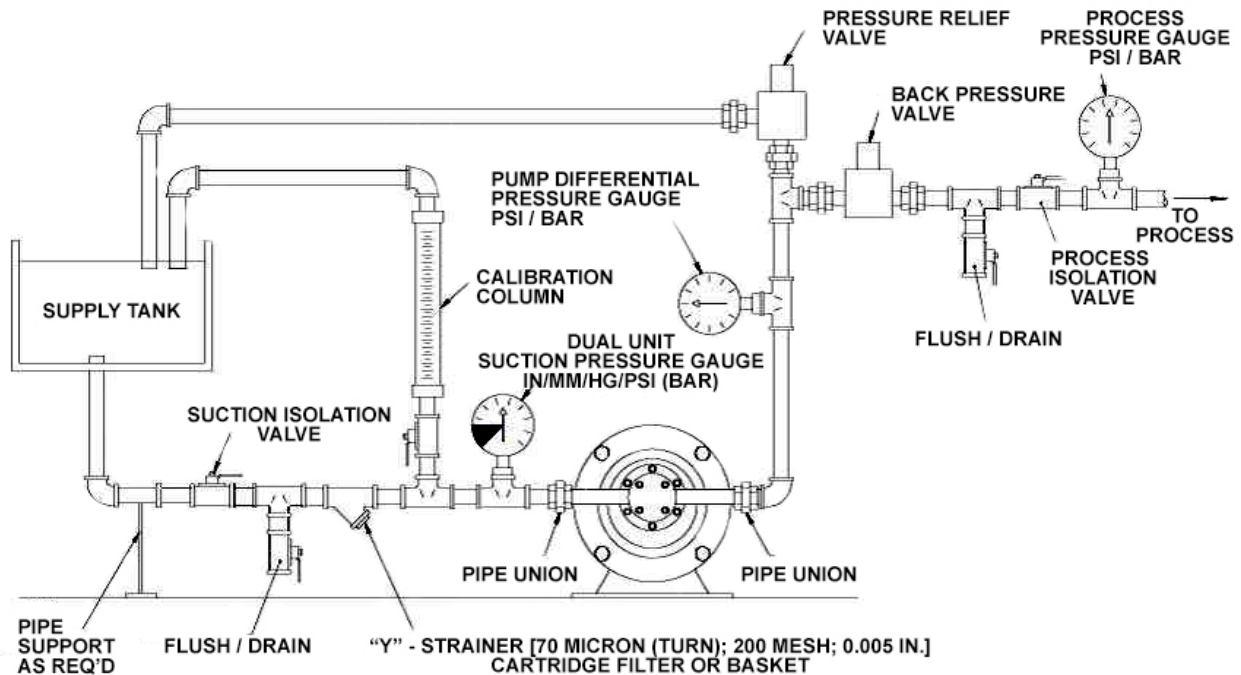
Figure 2a – General Installation
