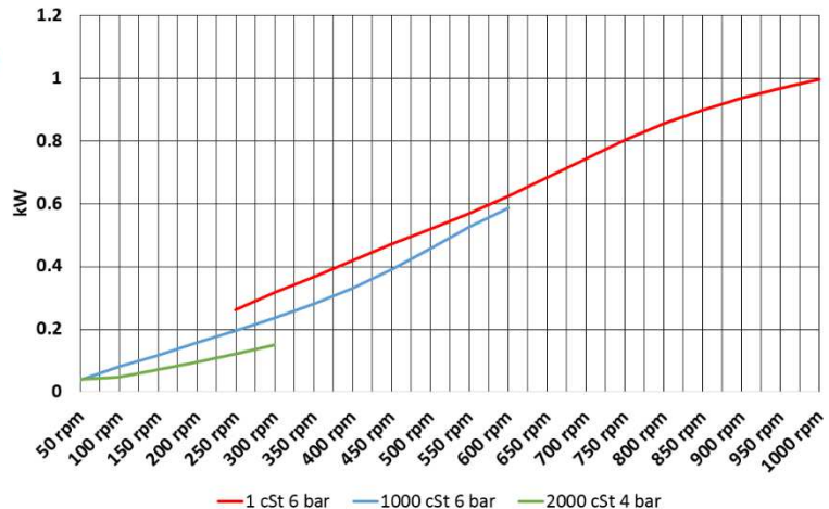
Absorbed power
