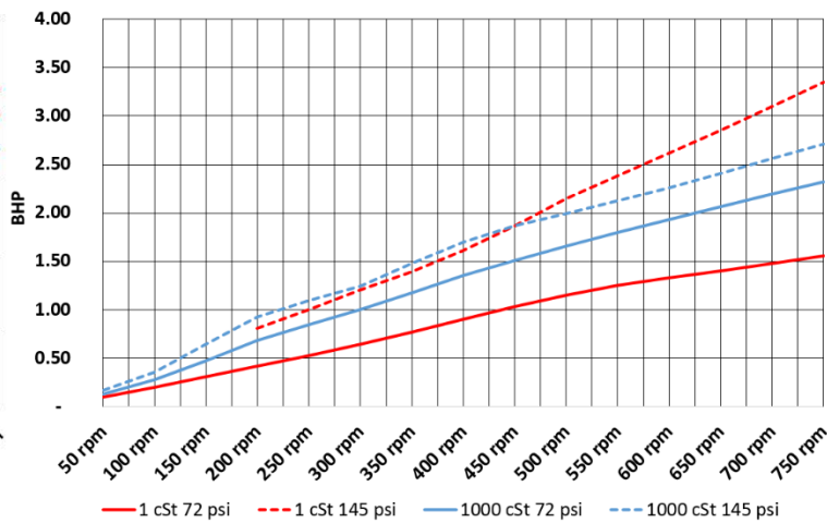
Absorbed power
