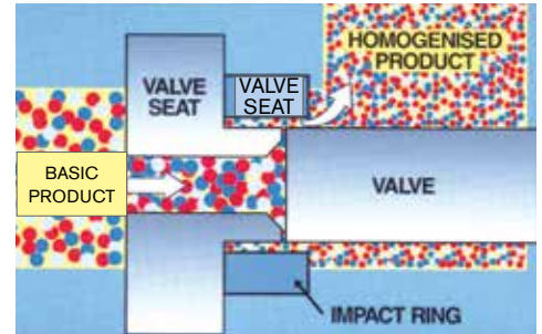
HOMOGENIZATION VALVE
