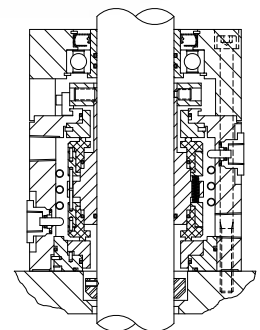
Double seal with integral bearing
