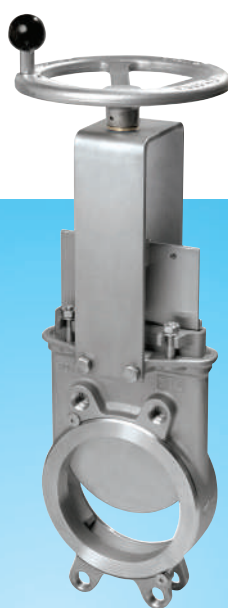
EK Unidirectional High Performance DN 50 – DN 1200 stainless steel
