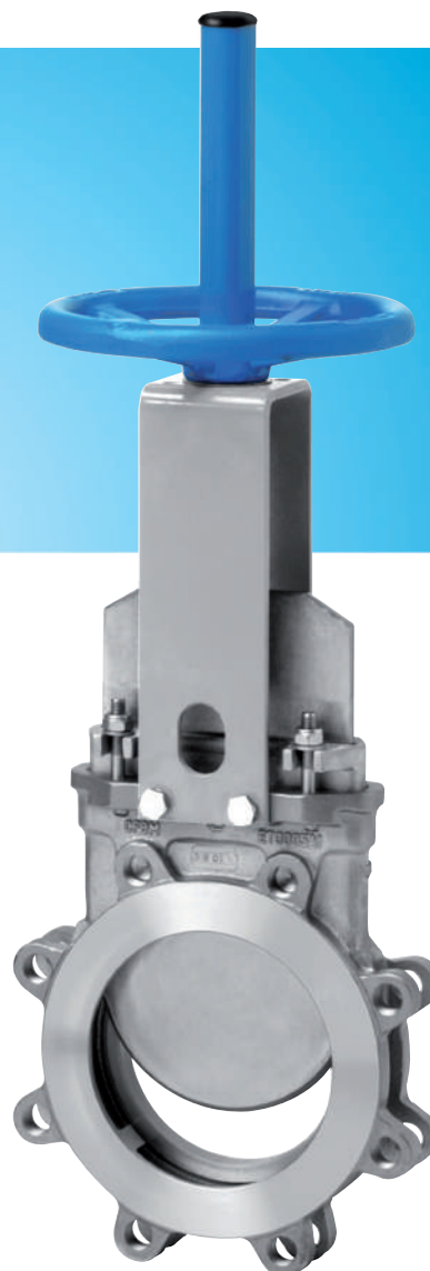
ET Unidirectional MSS SP-81 DN 50 – DN 900 stainless steel
