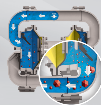
Bottom Discharge
